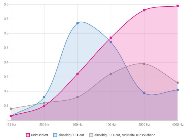
Schallabsorptionsgrad \alpha_s - Melaminharzschaumstoff t=20mm
